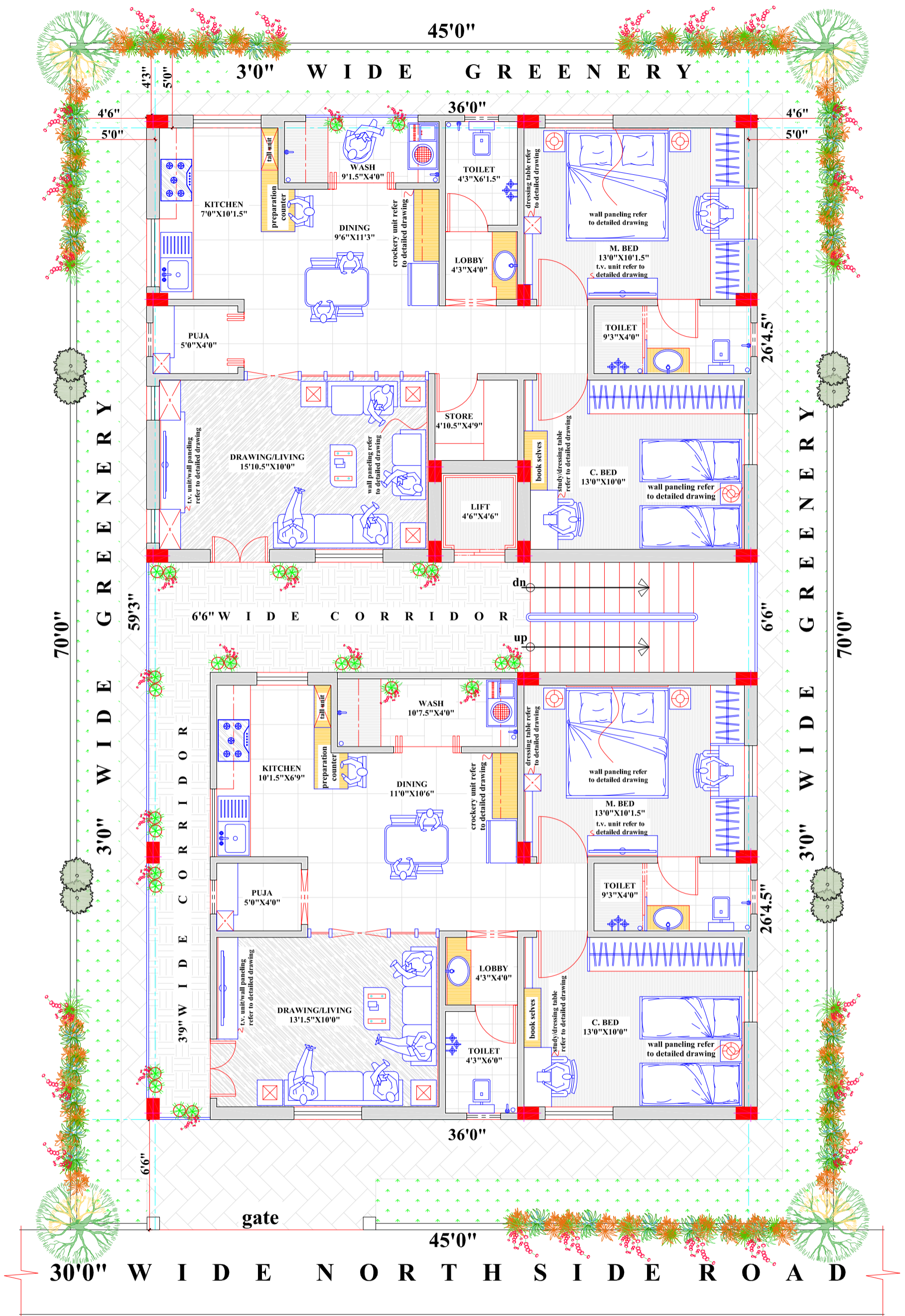
TYPICAL FLOOR PLAN (Slab Area: 2133.00 Sq.Fts.)
